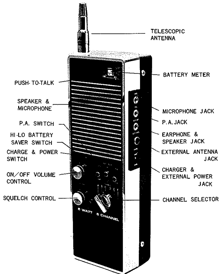
MODEL TNC-50 6 5 WATT 6 CHANNEL TRANSCEIVER
